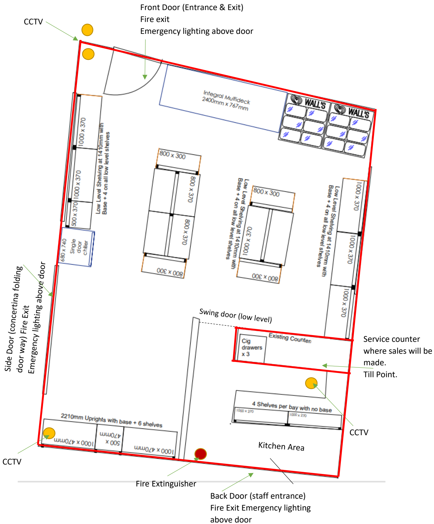
ZONE A – Shop Layout
