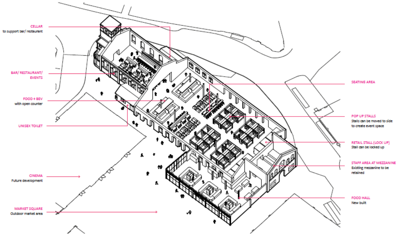
Axonometric view Group Ginger
